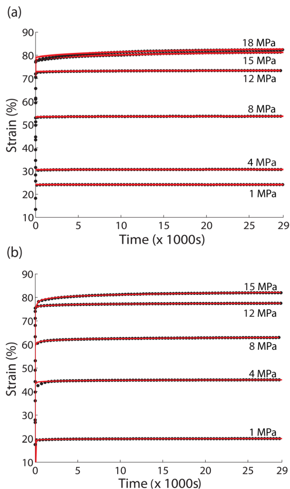
FIG. 2. Experimental creep response (points) and curve fitting (solid lines) of (a) freestanding and (b) double-anchored CNT forests.
