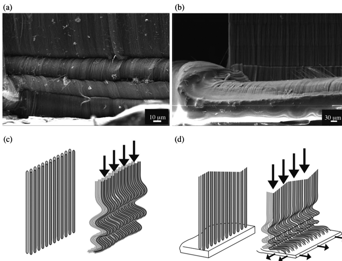
FIG. 5. Scanning electron microscope micrographs of the buckling area in the bottom section of (a) freestanding and (b) double-anchored CNT forests while compressed at \varepsilon = 0.4 . Schematic illustration of the different buckling mechanisms in (c) freestanding and (d) double-anchored CNT forests.
